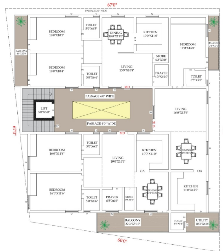
FIRST & SECOND FLOOR PLAN
